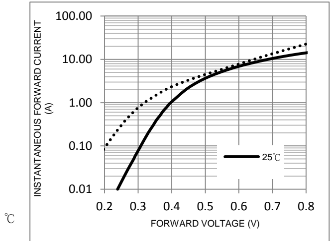
FIG. 2-Typical Forward Characteristics
