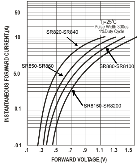
FIG.2-TYPICAL FORWARD CHARACTERISTICS
