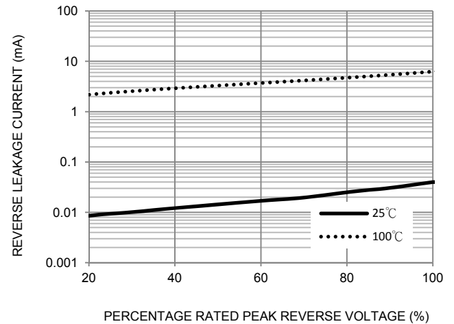
FIG. 4-TYPICAL REVERSE CHARACTERISTICS
