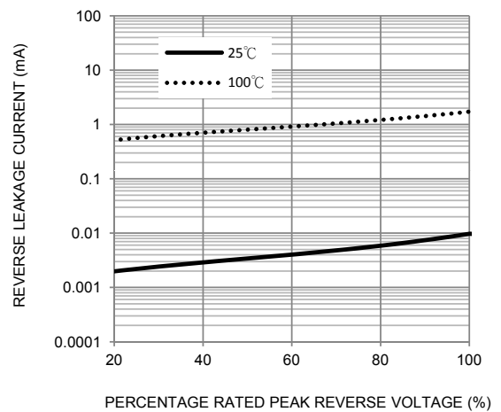
FIG. 4-TYPICAL REVERSE CHARACTERISTICS
