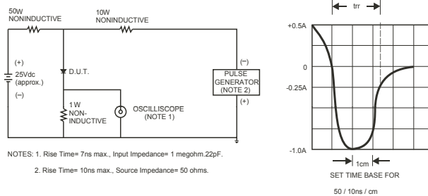
FIG. 6-Reverse Recovery Time Characteristic and Test Circuit
