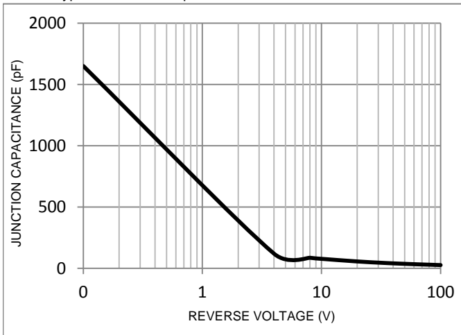
FIG. 5-Typical Junction Capacitance
