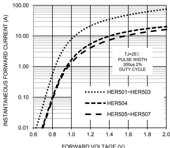
FIG. 2-TYPICAL FORWARD CHARACTERISTICS
