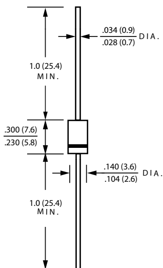
DO-15
